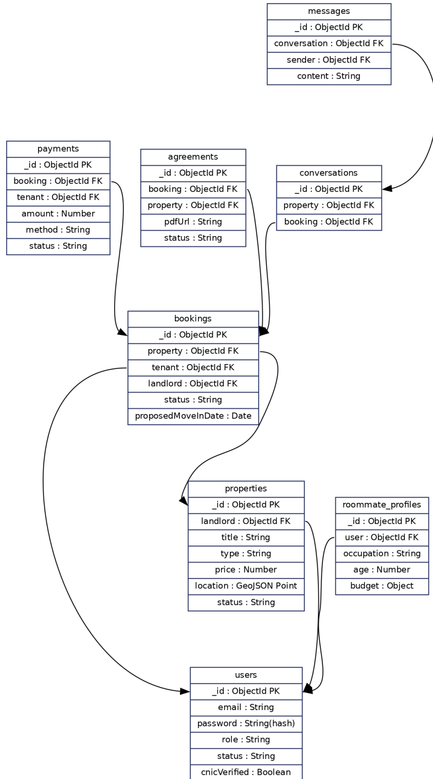
Figure 4.11: Database Schema Diagram (Sample)
