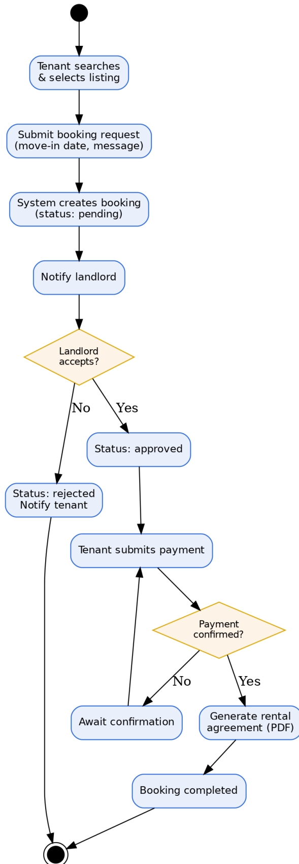
Figure 4.3: Activity Diagram (Sample)
