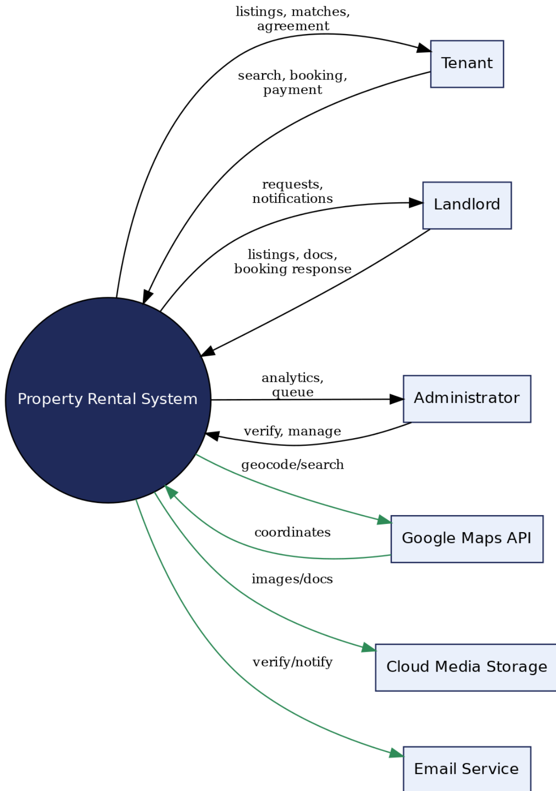
Figure 4.1: Context Diagram of the Property Rental System Platform
