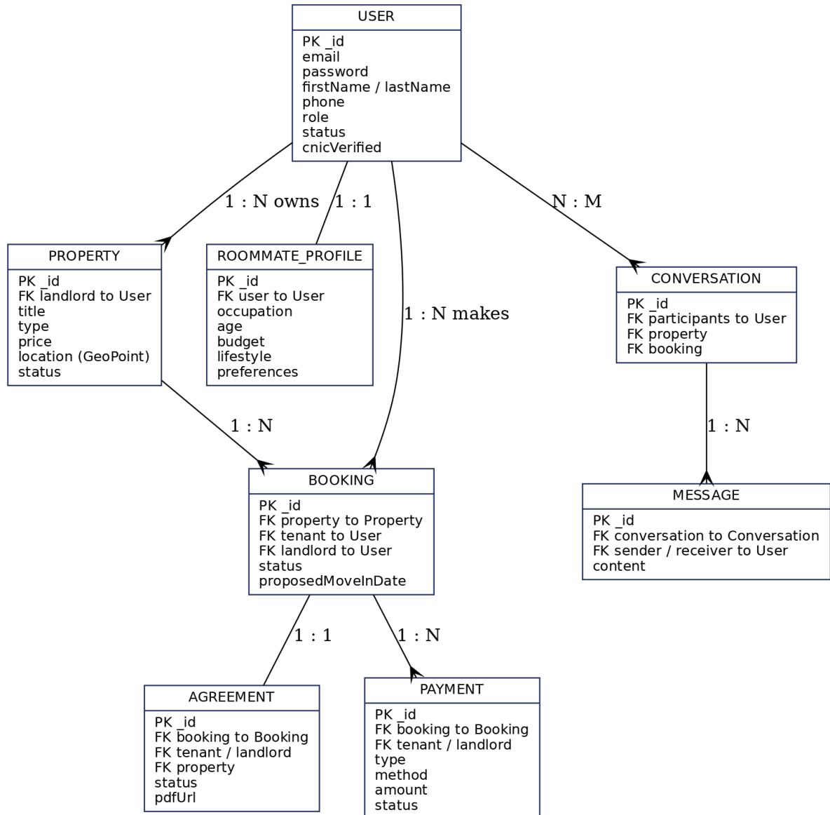
Figure 4.10: Entity Relationship Diagram (Sample)
