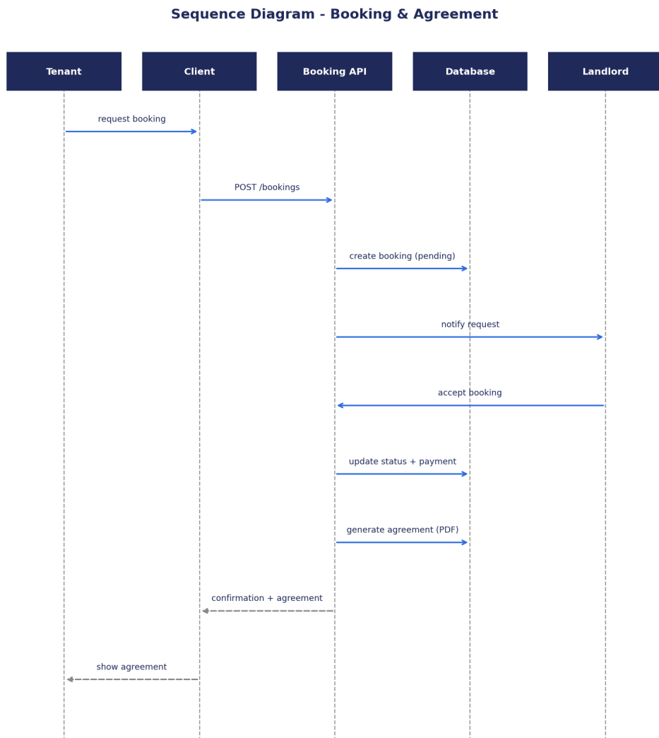
Figure 4.6: Sequence Diagram – Booking and Agreement (Sample)
