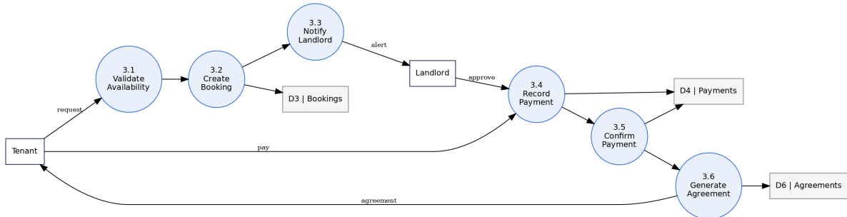
Level 2 DFD - Booking & Payment Process
