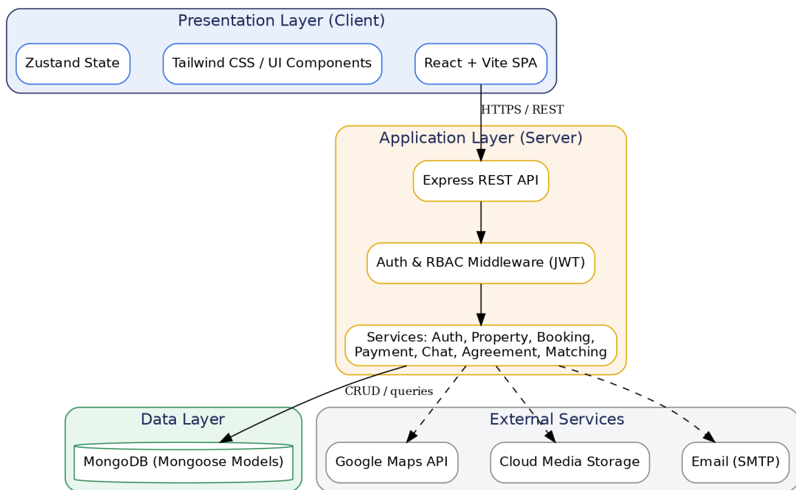
Figure 4.2: System Architecture of the Property Rental System Platform
