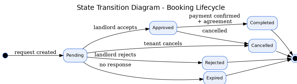
Figure 4.7: State Transition Diagram (Sample)
