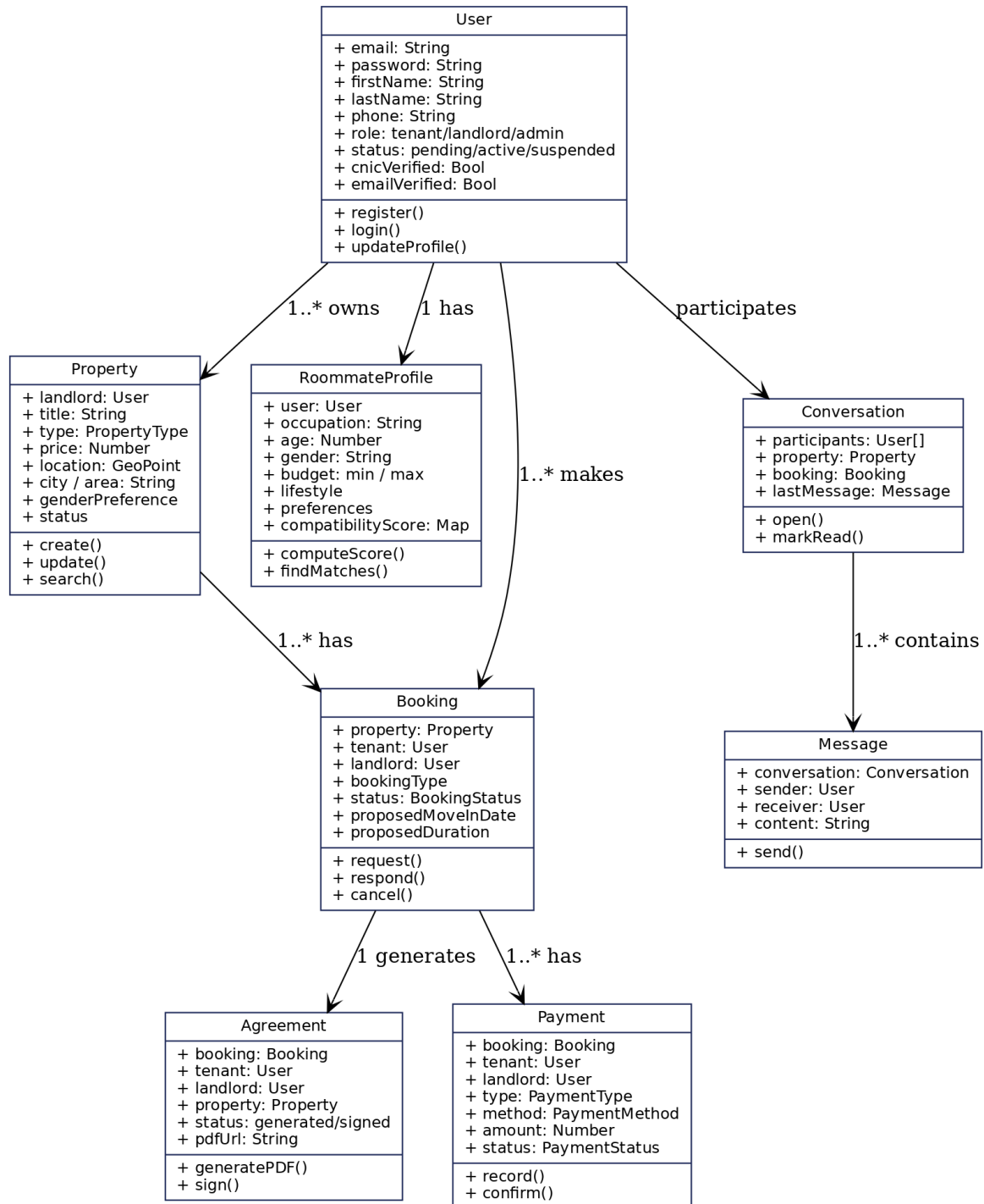
Figure 4.4: Class Diagram (Sample)
