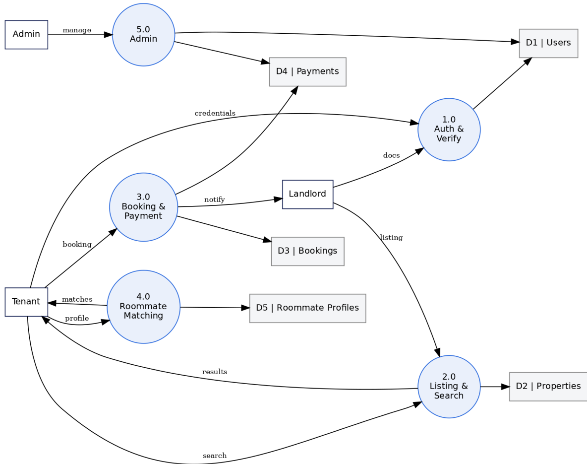
Level 1 Data Flow Diagram - Property Rental System
