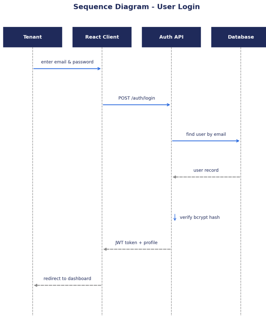
Figure 4.5: Sequence Diagram – User Login (Sample)
