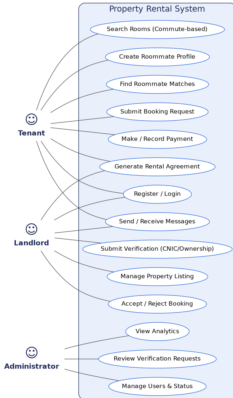
Figure 3.1: Use Case Diagram of the Property Rental System Platform
